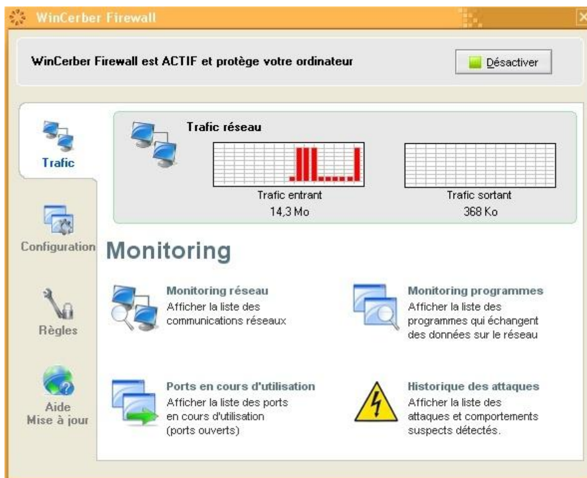
WinCerber Firewall
